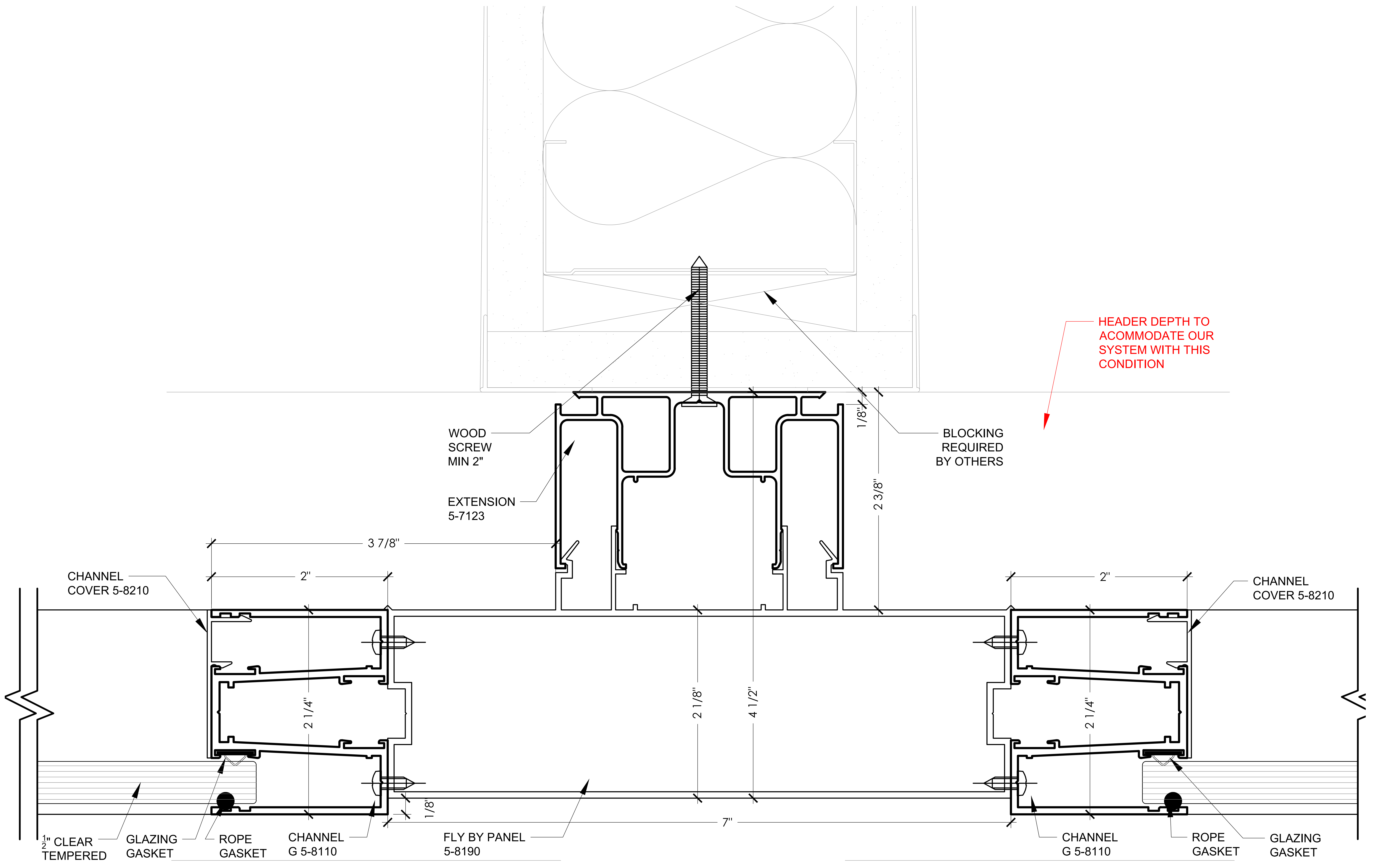
1 FLYBY DETAIL W/ GLASS PANELS Scale: 1'=1'
