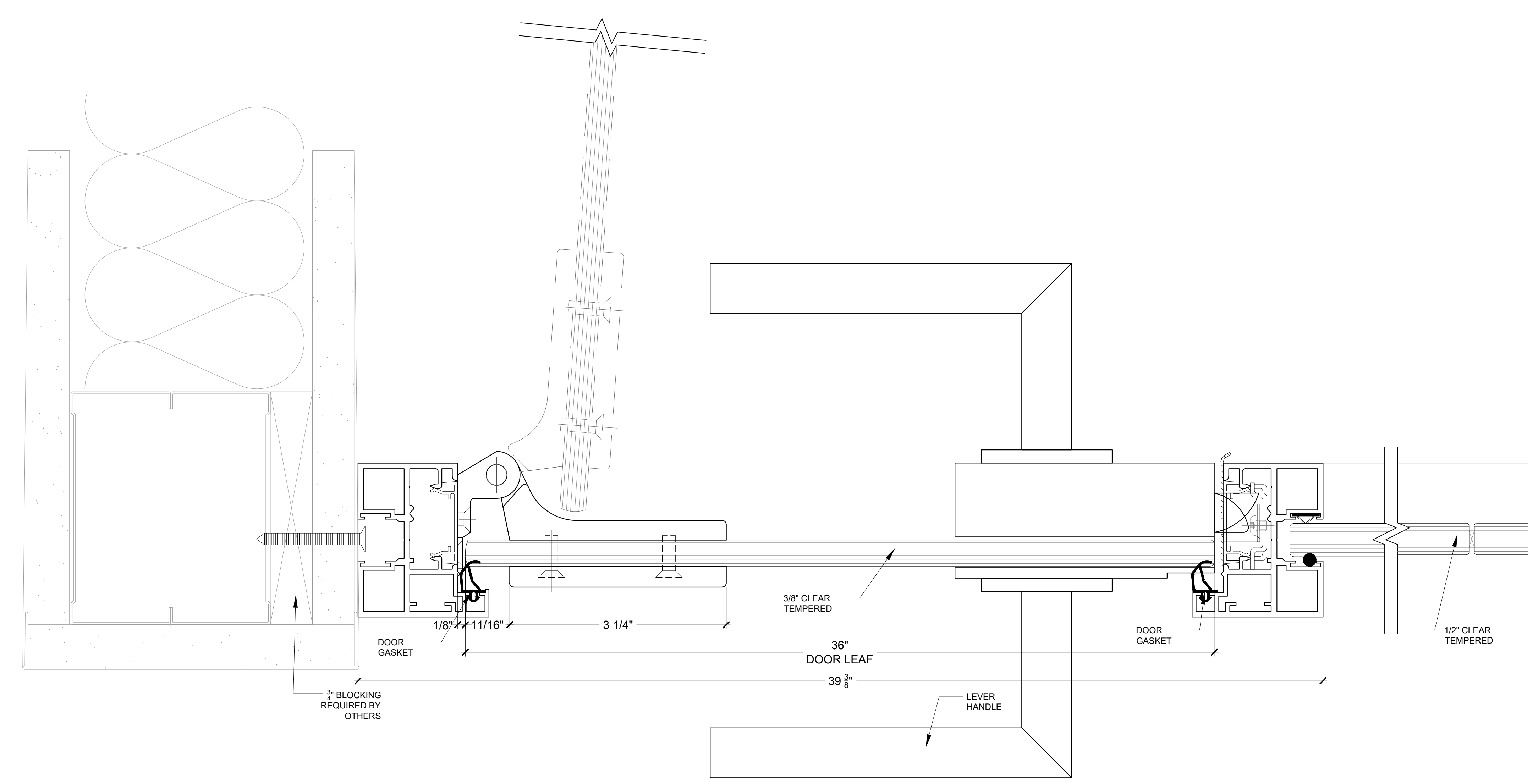
3 FRAMELESS HINGED CENTERED PIVOT DOOR W/ LEVER HANDLE 1'-0"=1'-0"
