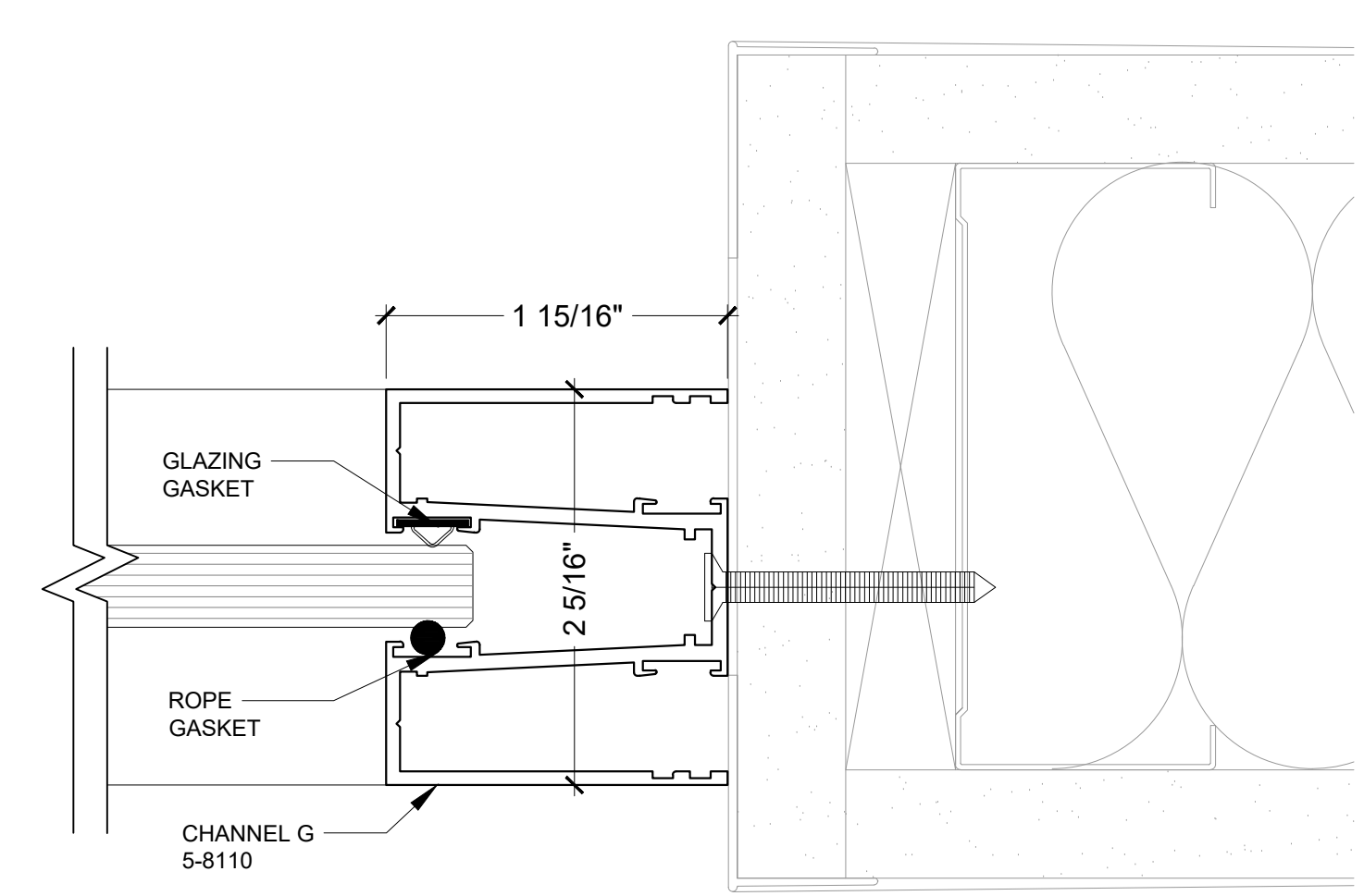
5 WALL ABUTMENT 1'-0"=1'-0"
