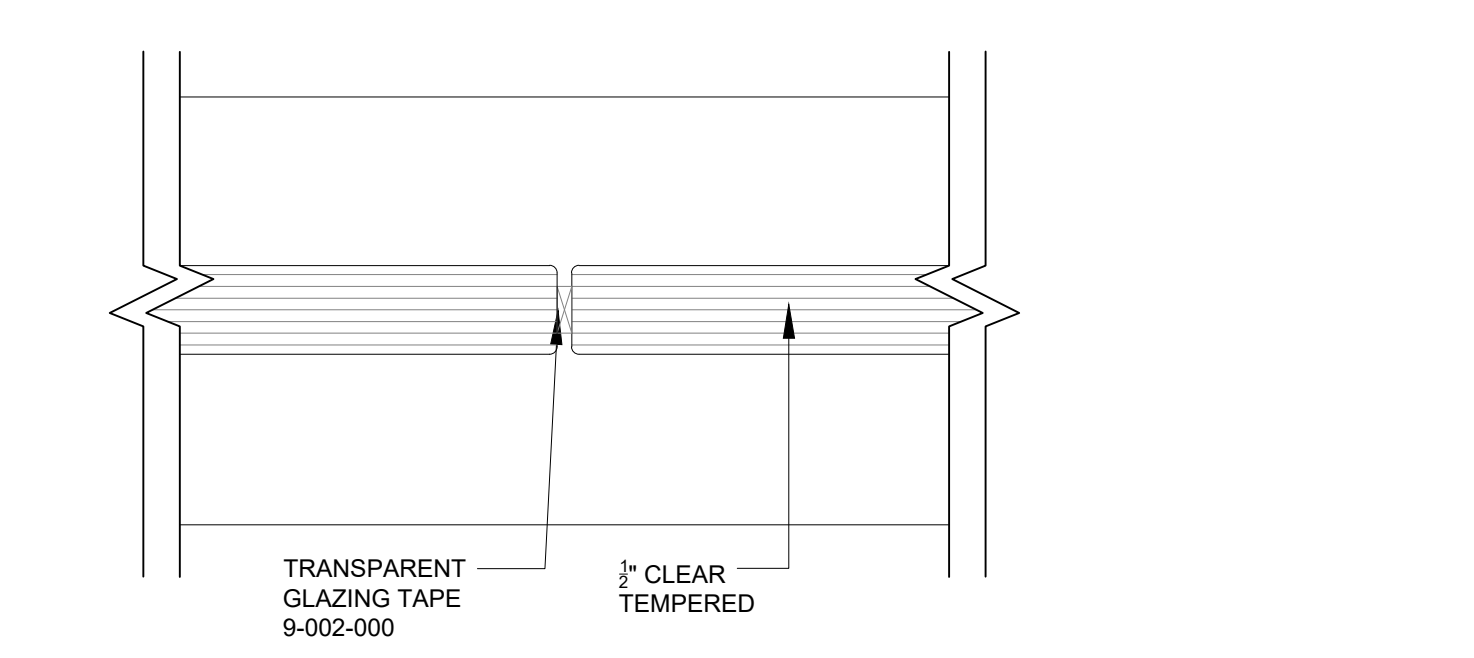
4 GLASS CONNECTION 1'-0"=1'-0"
