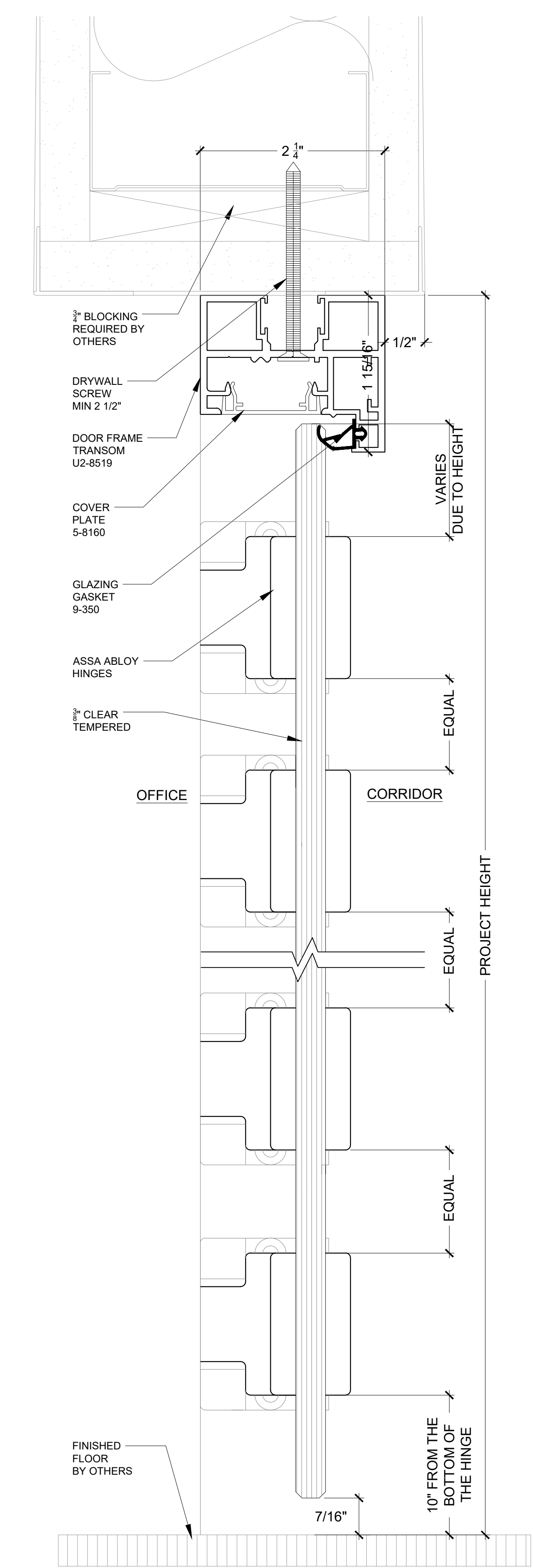
1 ELEVATION FRAMELESS HINGED PIVOT DOOR W/LEVER SCALE: 1/2"=1'-0"
