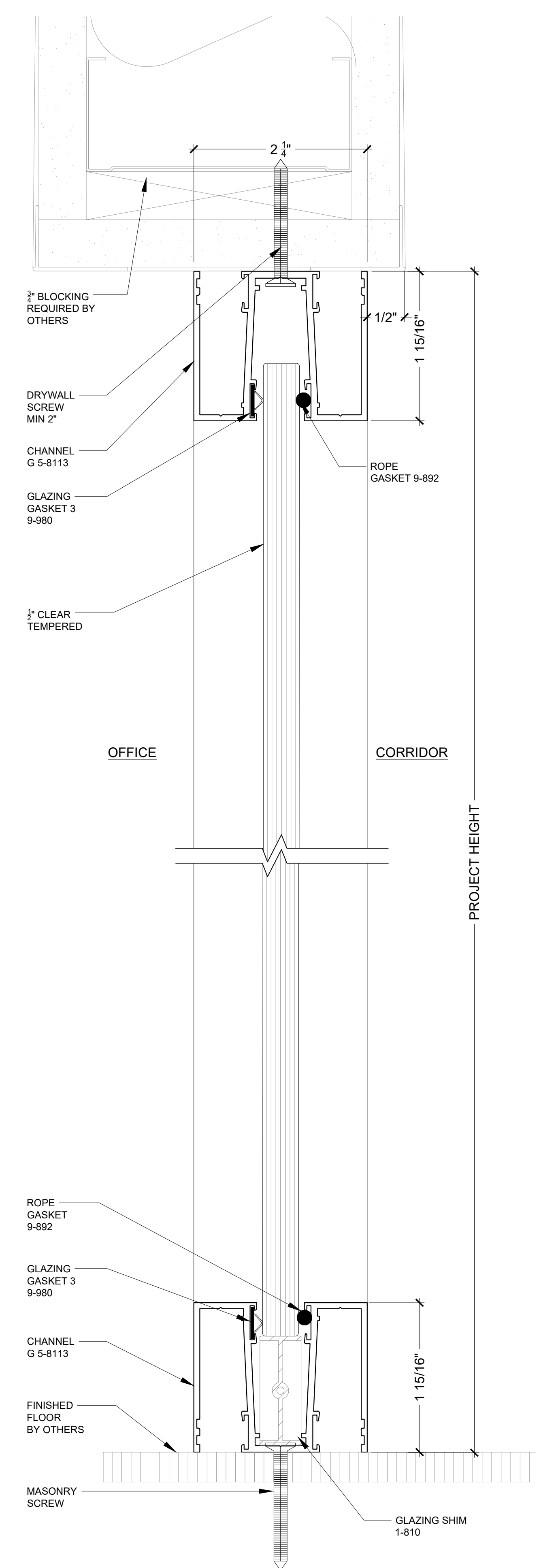
2 CENTERED FIXED CHANNEL 1'-0"=1'-0"
