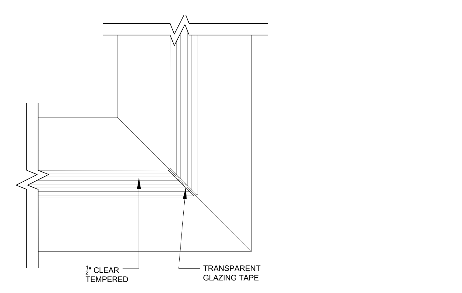
6 GLASS CORNER 1'-0"=1'-0"
