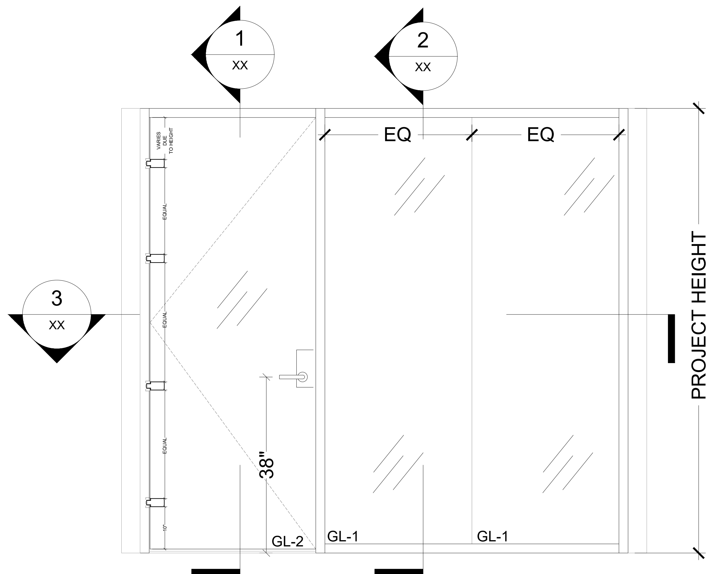
1 ELEVATION FRAMELESS HINGED PIVOT DOOR W/LEVER SCALE: 1/2"=1'-0"
